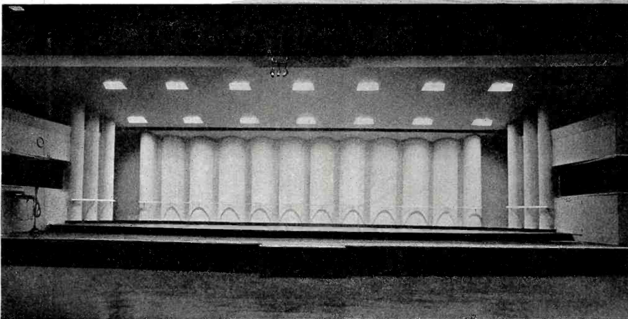
Above: Stage of NBC's studio 8-H. This is one of several studios provided with polycylindrical sound diffusers in order to obtain improved high-frequency response. All of these studios use RCA 44-BX Microphones (on stage), and RCA 77-B Microphones (suspended from ceiling).
